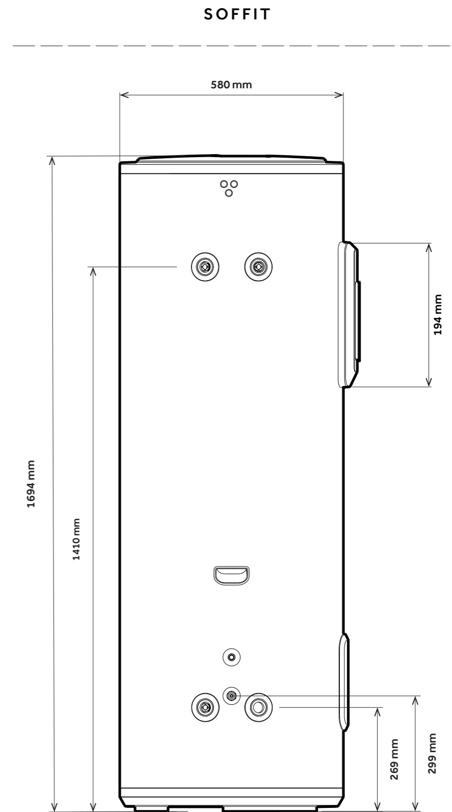
SIDE VIEW
